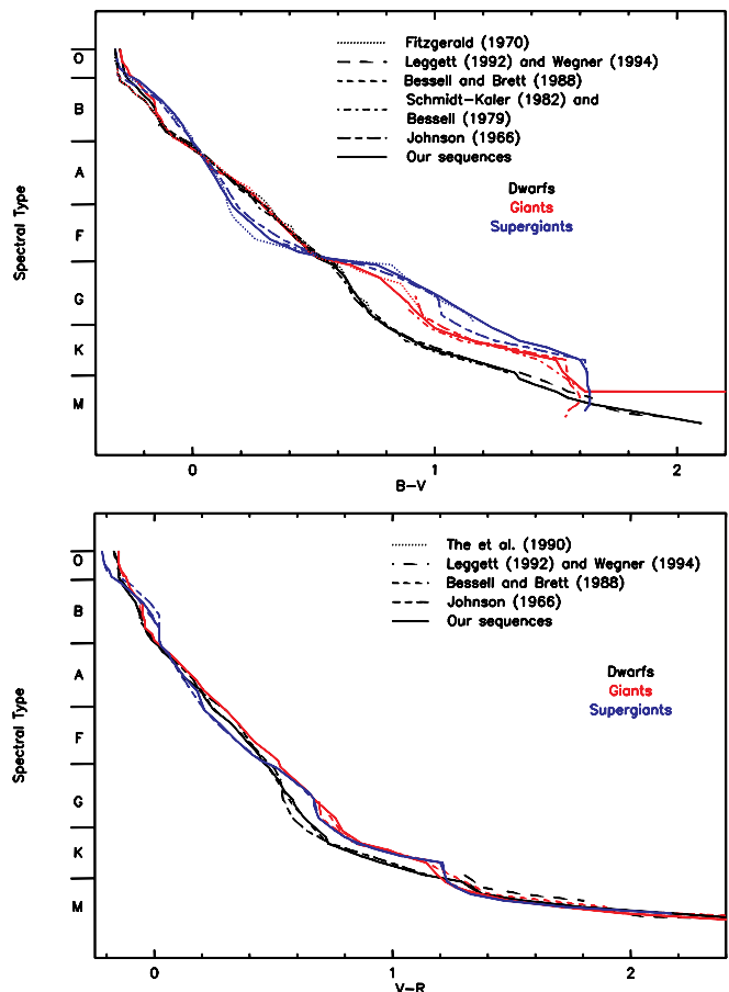
Fig. 1. Example of our “spectral type–luminosity class–color” relations used to compute missed photometry. The relation for dwarfs, giants and supergiants are shown in dark, red, and blue, respectively. Our sequences are plotted in solid lines, when the relation from which they are extracted are in different dashed lines.
