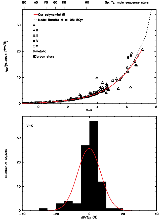
Fig. 3. top: \psi_V as a function of (V - K) color. The red line is our polynomial fit. bottom: Distribution of the angular diameters (O–C) from the \psi_V versus (V - K) colors relation. The red curve is a Gaussian function fitting the distribution of the (O–C). \Delta\theta is the difference between angular diameters computed from our relation and measured angular diameters
