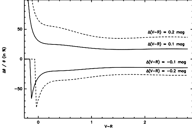
Fig. 4. Error in the determination of the angular diameter when the \psi_V versus (V - R) relation is used and when the (V - R) color have errors of -0.2 , -0.1 , 0.1 , and 0.2 mag.
