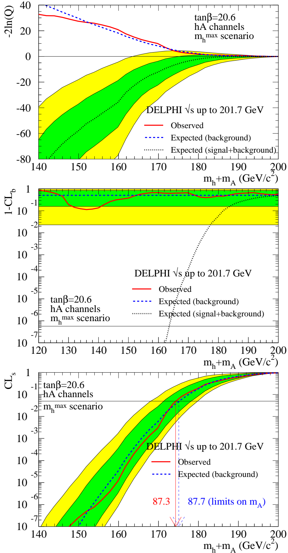
Figure 15: hA analyses: test-statistic (top) and confidence levels in background hypothesis (middle) and in signal hypothesis (bottom) as functions of m_h+m_A . Curves are the observed (solid) and median expected (dashed) confidences from background-only ex-
