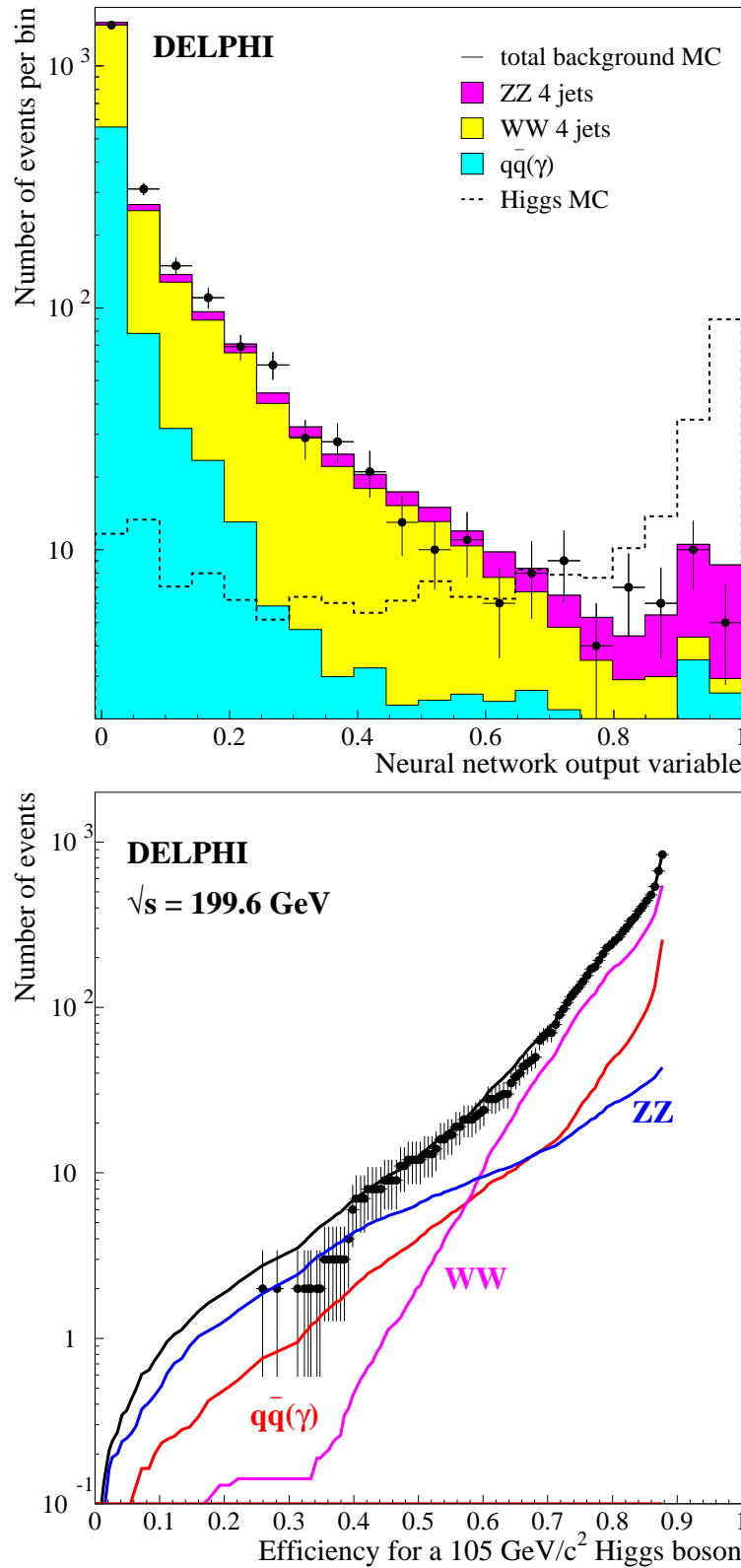
Figure 8: Hq\bar{q} channel: Top: distributions of the neural network variable for the expected SM backgrounds (full histograms), 191.6-201.7 GeV data (dots) and the expected Higgs signal at 105 GeV/c 2 (dashed histogram, normalised to 20 times the expected rate). Bottom: curve of the expected SM background rate at \sqrt{s} = 199.6 GeV as a function of the efficiency for a 105 GeV/c 2 Higgs signal when varying the cut on the neural network variable. The different colored lines correspond to the different SM backgrounds. The
