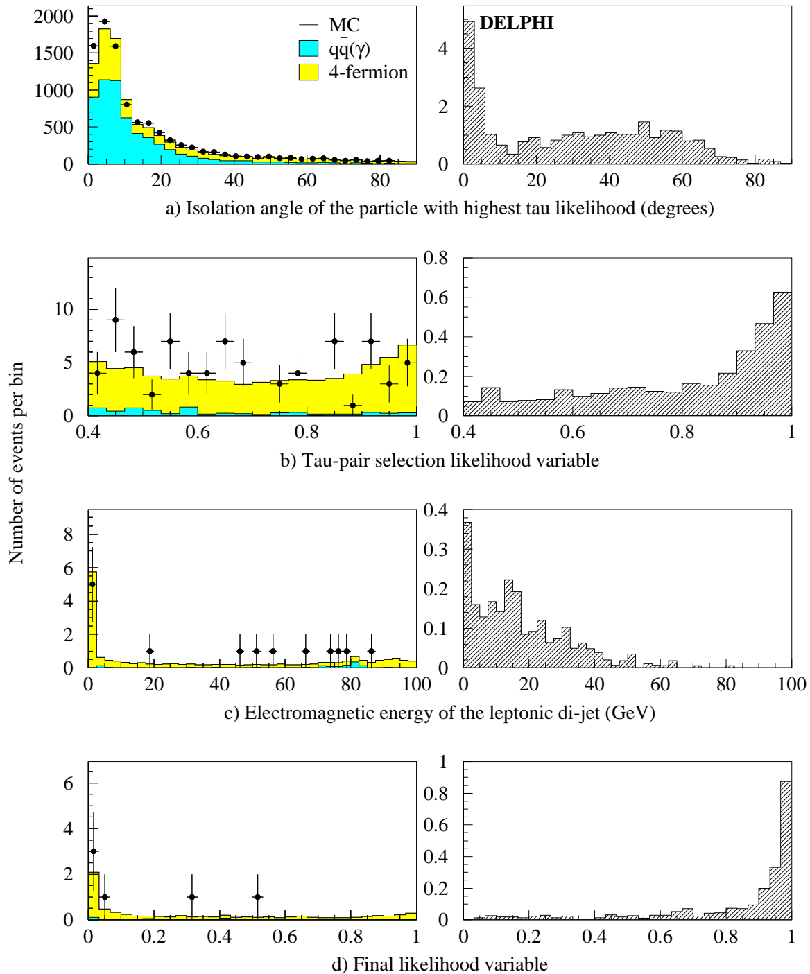
Figure 4: \tau^+\tau^-\bar{q}q channel: distributions of four analysis variables at different levels of the selection, as described in the text. Data at \sqrt{s} = 191.6\text{-}201.7 GeV (dots) are compared with SM background expectations (left-hand side histograms) and with the expected distribution for a 105\text{ GeV}/c^2 signal in the (h \rightarrow \tau^+\tau^-)(Z \rightarrow q\bar{q}) (right-hand side histogram, normalised to one hundred times the expected rate).
