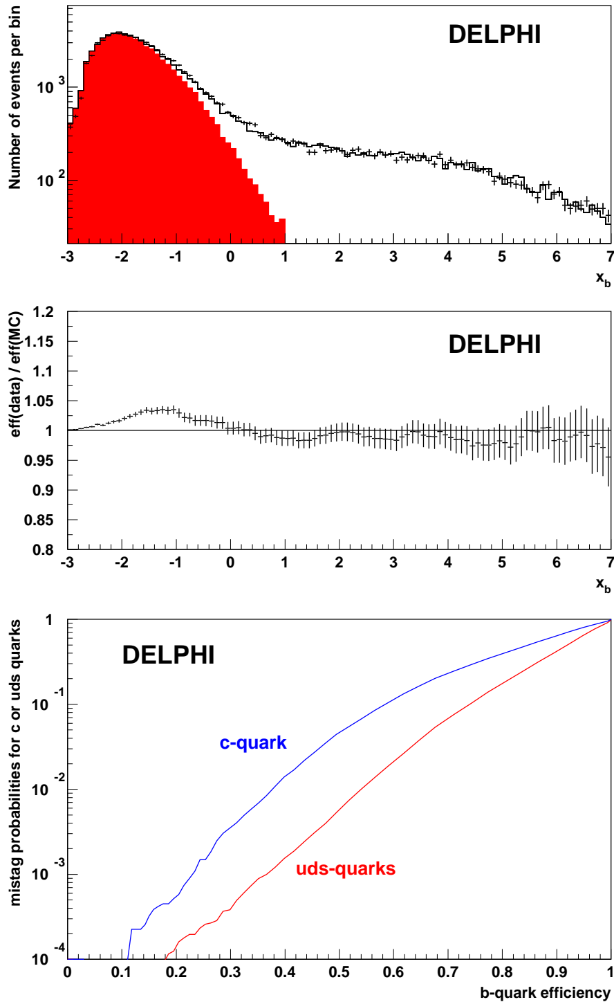
Figure 1: b-tagging: Top: distributions of the combined b-tagging variable x_b , in 1999 Z data (dots) and simulation (histogram). The contribution of uds-c-quarks is shown as the dark histogram. Middle: ratio of integrated tagging rates in Z data and simulation as a function of the cut in x_b . Bottom: mistag probabilities for c or uds-quarks as a function of the efficiency for b-quarks, estimated from simulated Z data.
