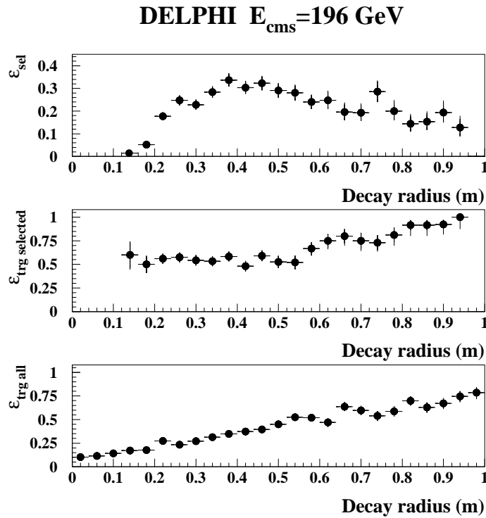
Figure 33: On top: efficiency for selecting a single 75 \text{ GeV}/c^2 chargino in the search for displaced decay vertices (kinks) at the centre-of-mass energy of 196 \text{ GeV} , as function of its decay radius. In the middle: trigger efficiency for the selected charginos. Below: trigger efficiency for all 75 \text{ GeV}/c^2 charginos, whether or not they were selected.
