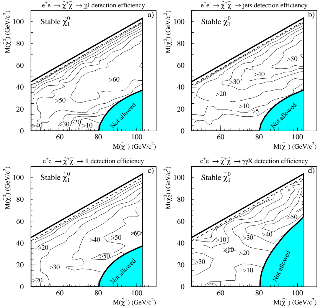
Figure 26: Chargino pair production detection efficiencies (%) for the four decay channels a) jjl , b) jets , c) ll and d) rad , at 206 GeV in the (M_{\tilde{\chi}^\pm}, M_{\tilde{\chi}^0}) plane. TPC sector 6 on and a stable \tilde{\chi}_1^0 are assumed. The shaded areas are disallowed in the MSSM scheme.
