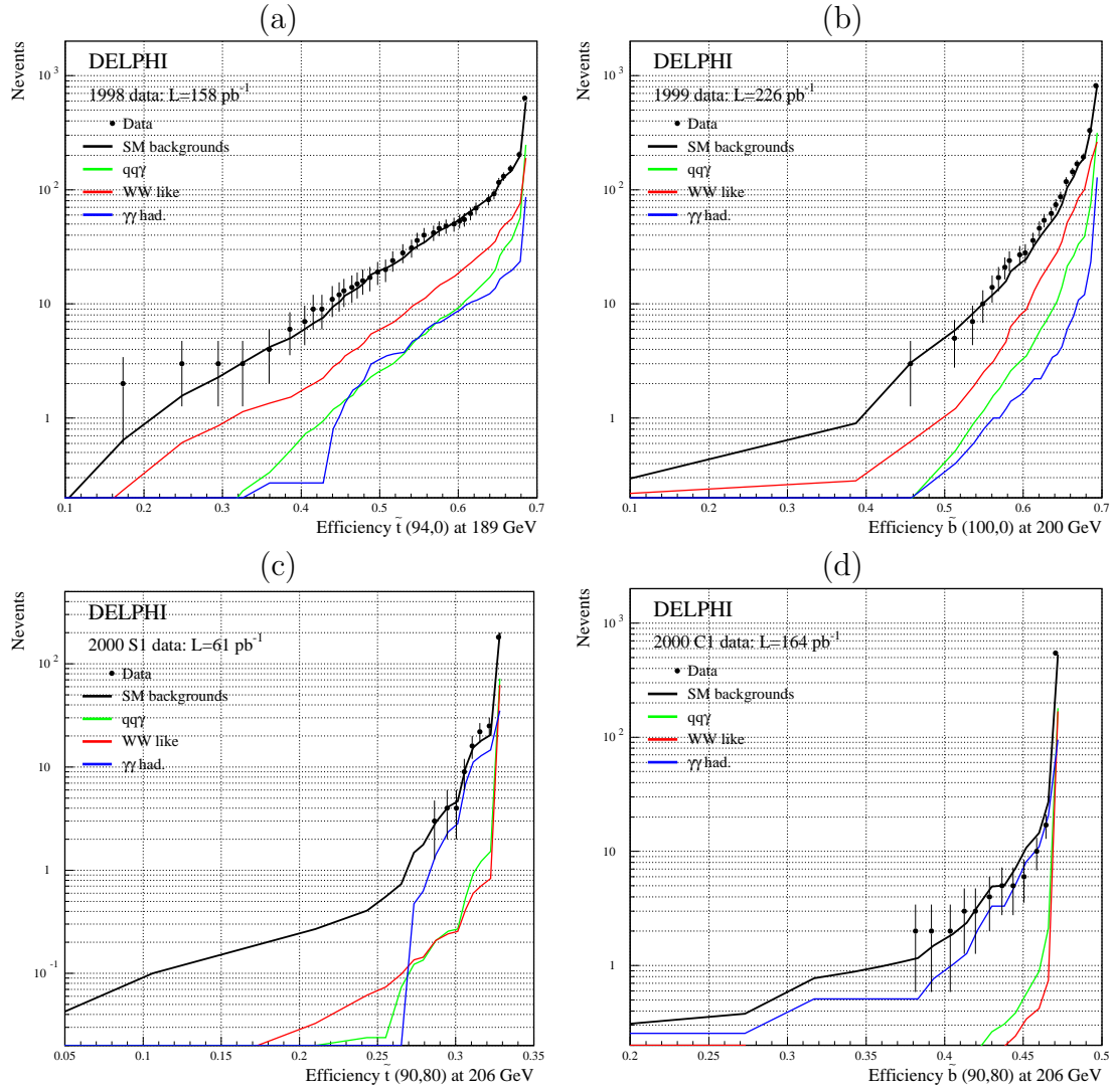
Figure 5: Number of events as a function of the signal detection efficiencies in the non-degenerate squark analysis: (a) 1998 data at 189 GeV: stop analysis for \Delta M > 20 GeV/c 2 , (b) 1999 data from 192 to 202 GeV: sbottom analysis for \Delta M > 20 GeV/c 2 , (c) 2000 data with TPC sector 6 off: stop analysis for 5 \leq \Delta M \leq 20 GeV/c 2 , (d) 2000 data with TPC sector 6 on: sbottom analysis for 5 \leq \Delta M \leq 20 GeV/c 2 .
