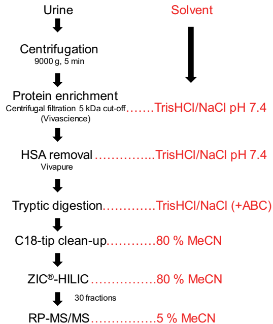
Figure 9. Schematic outline of the main steps of the method workflow and solvents used in the respective steps.
