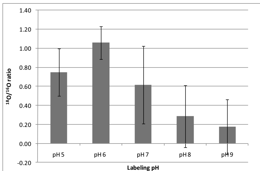
Figure 18. Average ^{18}\text{O}/^{16}\text{O} -ratios ( \pm SD) of 12 BSA / cyt c peptides using labeling buffer of pH 5, 6, 7, 8 or 9 ( n = 3 ). Reaction time was 2 hours for all samples
