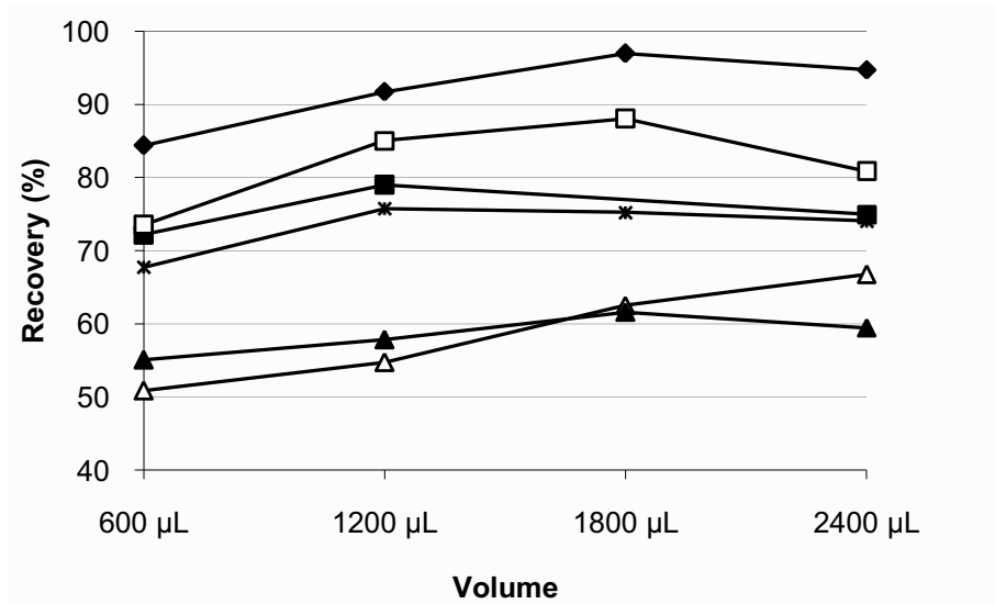
Figure 10. Protein recovery from centrifugal filters (5 kDa cut-off) using different volumes of water (×), 25 mM TrisHCl (▲), 25 mM TrisHCl + wash (Δ), 8 M Urea (◆), 10 mM TrisHCl/150 mM NaCl (■), 10 mM TrisHCl/150 mM NaCl + wash (◻) to redissolve the proteins after centrifugation
