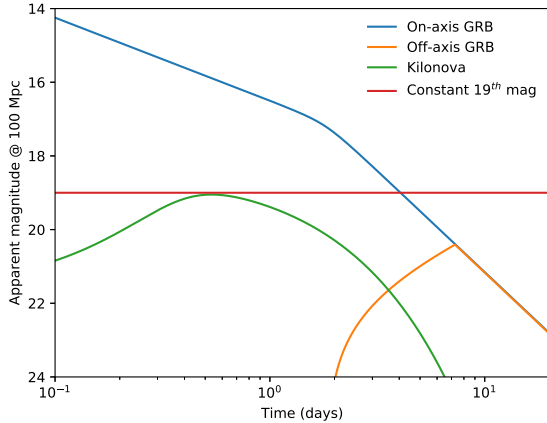
Figure 1. Light curves of our test sources at an assumed distance of 100 Mpc.
