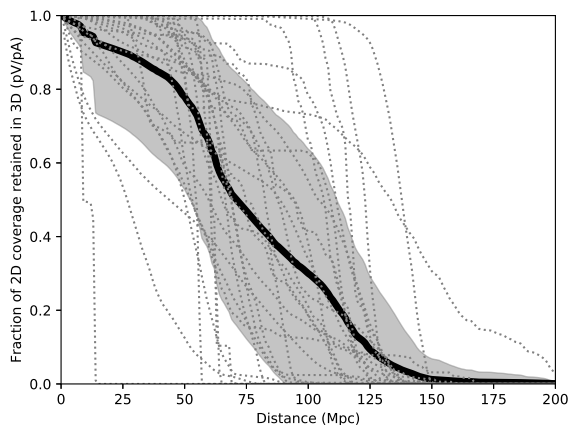
Figure 5. The fraction of the 2D probability coverage that is retained with increasing distance. Each dotted line represents an LVC follow-up campaign with GOTO-4. The thick black line is the mean of the 29 events, and the grey area is the 1\sigma standard deviation.
