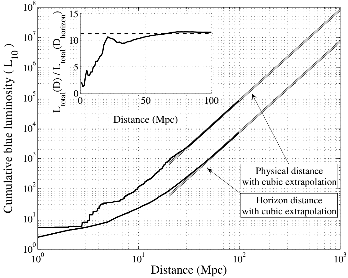
Figure 3.6: Cumulative luminosity as a function of physical distance (top line) and horizon distance (bottom line). The horizon distance D_{\text{horizon}} is defined as the physical distance to an optimally oriented and located binary system that would be detected with a signal-to-noise ratio of 8. (Instrumental sensitivity range is sometimes quoted in terms of the radius of a sphere with the same volume as the non-uniform region probed by the instrument, this sensitivity range D_s is related to the horizon distance by D_s \simeq D_{\text{horizon}}/\sqrt{5} ). The gray shaded lines are cubic extrapolations (§3.3) derived for both cases. Given a LIGO horizon distance one can immediately get the cumulative blue luminosity from the bottom curve. To obtain an approximate rate upper limit one could calculate \mathcal{R}_{90\%} [\text{yr}^{-1} L_{10}^{-1}] = 2.3/(\mathcal{C}_L \times T) where \mathcal{C}_L is taken from this plot at a given range in horizon distance. Inset : Ratio of the cumulative luminosity for the physical and horizon distance from the completeness corrected CBCG-catalog illustrates the non-uniform distribution at smaller ranges ( < 20 Mpc) and asymptotes to the expected uniform distribution ratio (dashed line) for larger distances.
