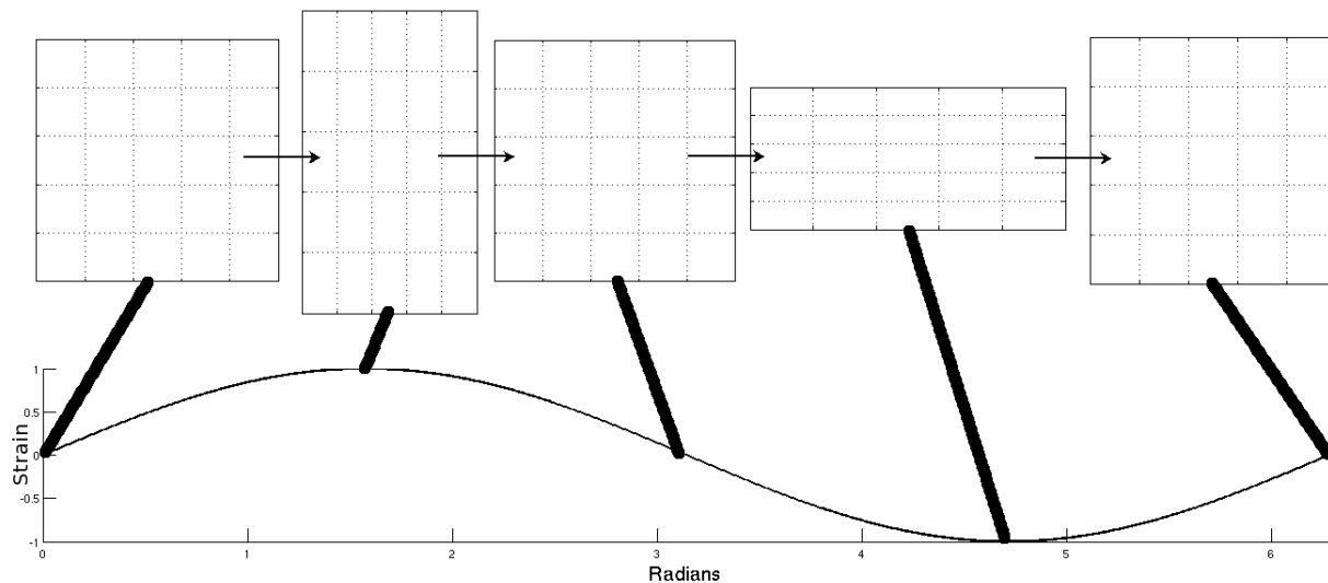
Figure 1.2: The effect of gravitational-waves on distances between points. This grid represents the metric on the 2 dimensional space of this page. As the gravitational-wave passes through the page the distances in the x and y directions of the grid shrink and expand. Gravitational-waves have two possible polarizations. Shown is the “plus” polarization. The “cross” polarization is rotated by 45^\circ . One would measure different distances between free masses in the path of a gravitational-wave depending on the time of the measurement. LIGO attempts to measure the time varying metric with a laser interferometer because the light output will be modulated by the strain as shown in the partial sinusoid below. (see next section).
