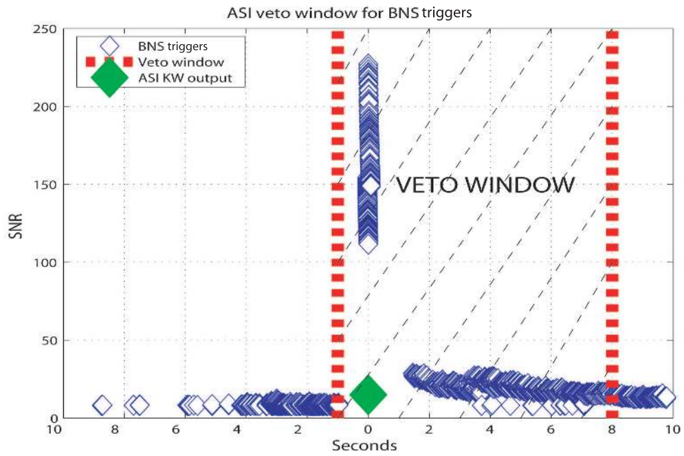
Figure 5.4: The SNR of BNS triggers found in the LIGO S3 data from H1, versus the time between the BNS trigger and the nearest Kleiweille ASI glitch trigger. The high SNR BNS triggers are coincident with the glitch found in the ASI channel. There is also a tail of lower SNR triggers at larger values of the time difference.
