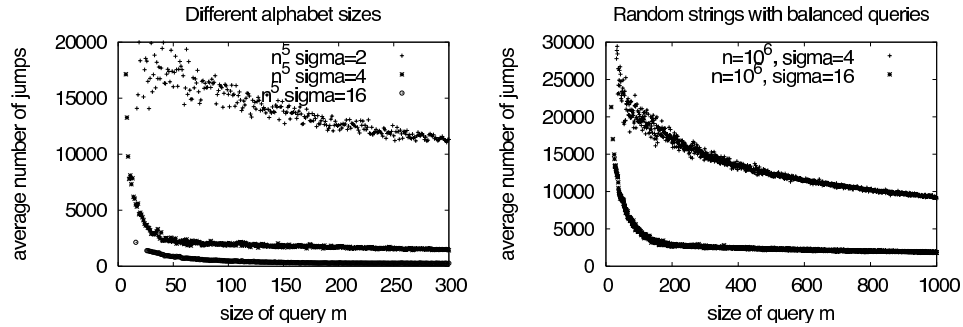
Figure 3. Number of jumps for different alphabet sizes for random strings of size 100000 (left) and 1000000 (right). All queries are randomly generated quasi-balanced Parikh vectors (cf. text). Data averaged over 10 strings and all random queries of same length.
