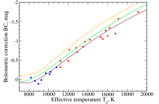
Fig. 1. Bolometric corrections using integrated fluxes of magnetic Ap stars from Lanz (1984, red circles), Stępień & Dominiczak (1989, blue circles), and Monier (1992, blue circles) as functions of effective temperature. The upper solid line is the BC for normal stars from Schmidt-Kaler (Lang 1992); the middle line is Balona’s (1994) fit to the fundamental data of Code et al. (1976) and Malagnini et al. (1986), and the lowest curve is a polynomial fit to the Ap data as described in the text.
