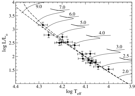
Fig. 2. Comparison of computed positions of stars in the Lower Centaurus-Lupus, Upper Centaurus-Crux, and Upper Sco regions of the Sco OB2 association with evolution tracks for stars of Z = 0.02 and M = 2, 2.5, 3, 4, 5, 6, 7, and 9 M_{\odot} , and with bracketting isochrones for log ages of 6.9 and 7.2, appropriate for these regions of the association.
