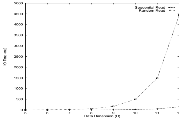
Figure 10: Sequential vs. Random IO Performance
