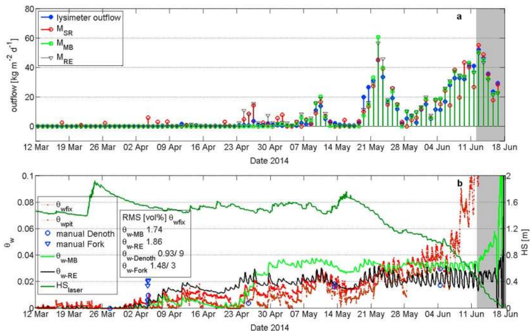
Figure 4. (a) Diurnal melt rates and (b) seasonal characteristics for \theta_w for the flat site WFJ in spring 2014. The gray shaded period represents dates when upGPR data are not reliable; for other notations see Figures 1 and 3.
