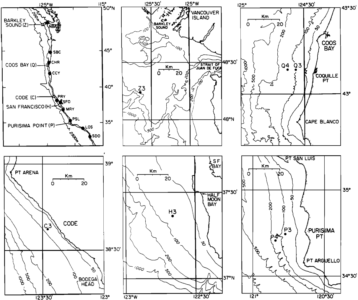
Fig. 1. The locations of the five mooring sites (open squares) and sea level data (solid circles) are shown at the top left. Details of the bathymetry around each mooring are shown in the other panels (isobath depths are in meters). Note the change in horizontal scale of the map for Z3 (48°N).
