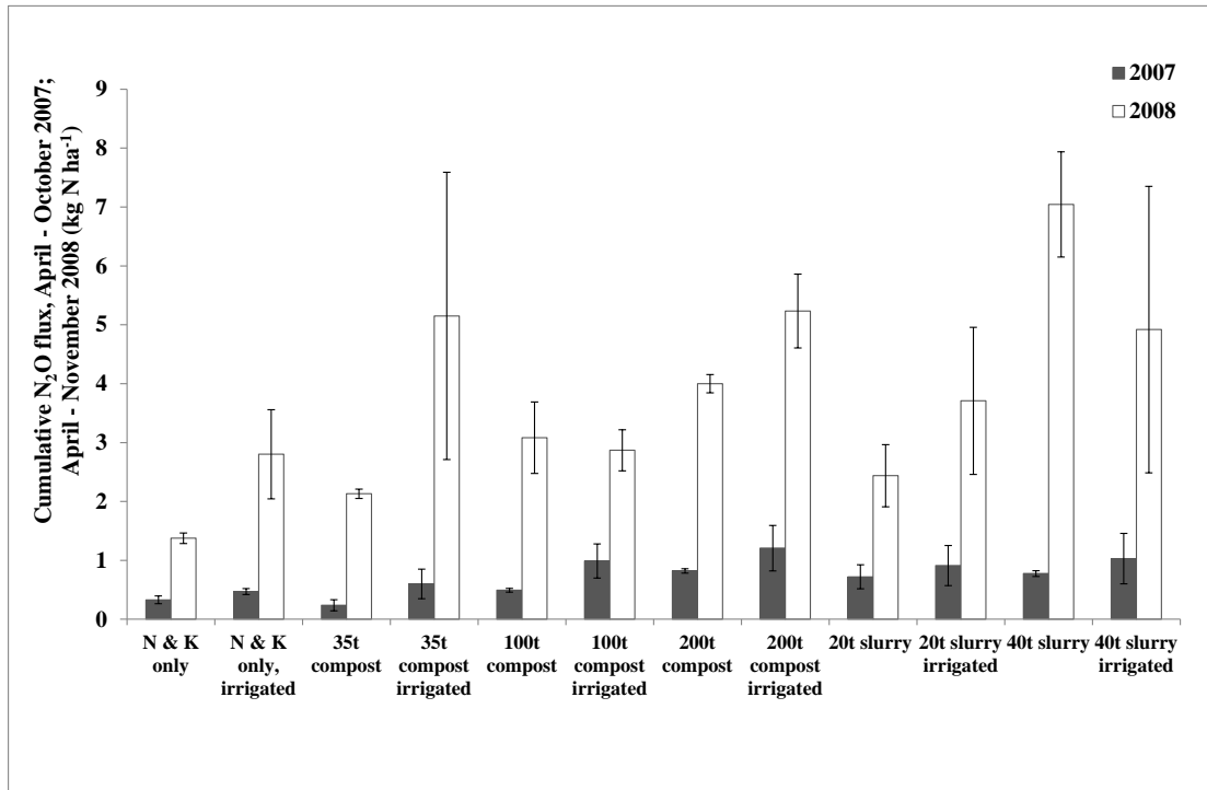
Figure 2 Cumulative N_2O emissions for 2007 and 2008 at the Amendment Experiment for (a) the control and residue treatments averaged over irrigation rates and (b) yearly totals for individual treatment combinations. For clarity, the error bars represent either plus or minus the standard error of the mean.
