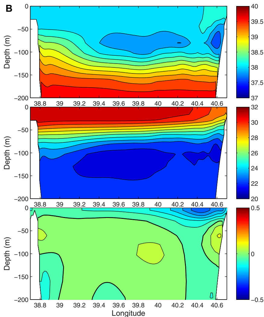
Figure 8b. Vertical sections of (top) salinity (psu), (middle) temperature ( ^{\circ}\text{C} ), and (bottom) cross-section velocity ( \text{m s}^{-1} ) at 18^{\circ}\text{N} , from the model data averaged in September 1980.
