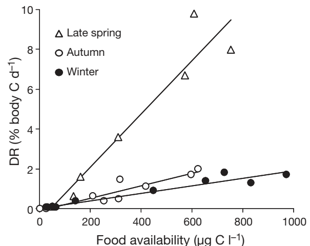
Fig. 4. Euphausia superba . Seasonal daily C ration (DR) as a function of food availability. Data points represent individual experiments. The seasonal linear regressions are shown in Table 7
