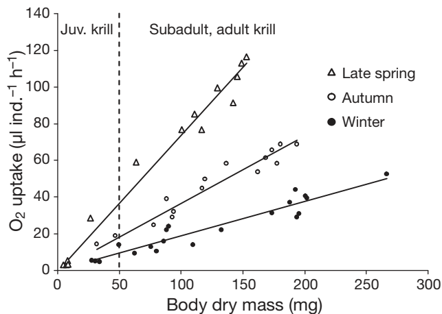
Fig. 8. Euphausia superba . Relationship of body dry mass and oxygen uptake rates of individual krill in different seasons. The linear regressions are shown in Table 7. Juvenile, subadult and adult krill were defined after Siegel (1987)
