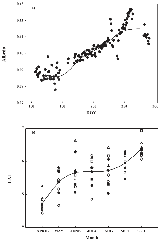
Figure 8. Changes in canopy properties during the entire observation period (16 April 1999 to 19 October 1999) at Caxiuana including (a) albedo, shown as the daily mean for data between 1100 and 1300 hours, and (b) leaf area index (LAI) per month at eight different locations around the tower. Different symbols represent each location. The monthly mean of the eight locations is shown as a spline curve.
