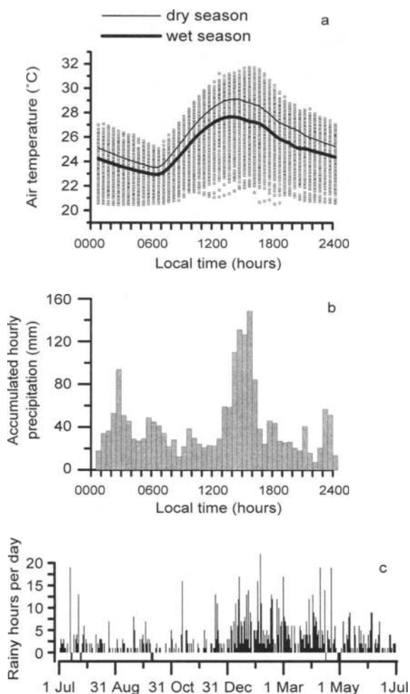
FIG. 2. (a) Diel pattern of air temperature at 64 m (30-min average). The thin solid line shows the dry season average (20 July–14 December 2000); the thick solid line shows the wet season average (1–13 July 2000 and 15 December 2000–30 June 2001). (b) Diel pattern of accumulated hourly precipitation. (c) Number of rainy hours per day (negative bars are missing values).
