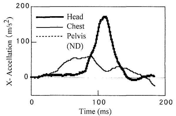
Figure 7A. \Delta V=12.5 dummy response (D11).
