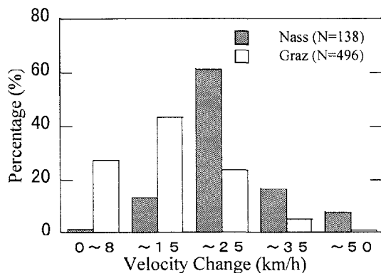
Figure 2. Distribution of velocity change ( \Delta V ) of the struck car in rear end collisions involving whiplash injury.
