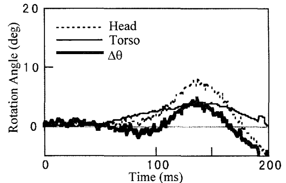
Figure 11. Volunteer response (V02).
