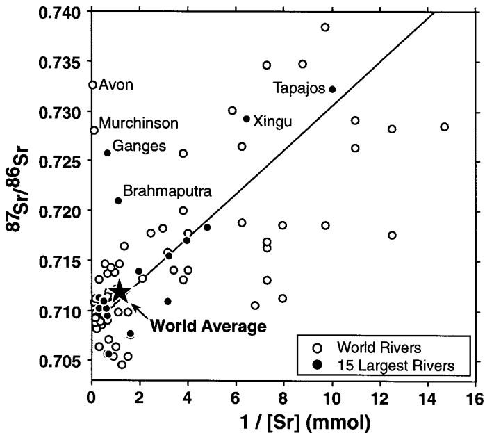
Fig. 7. The inverse relationship between 1/\text{Sr} and ^{87}\text{Sr}/^{86}\text{Sr} in rivers largely reflects rivers draining ancient granitic terrains (low Sr concentrations, ^{87}\text{Sr}/^{86}\text{Sr} > \sim 0.715 ) versus rivers that include Phanerozoic limestones in their drainages (highest Sr concentrations, ^{87}\text{Sr}/^{86}\text{Sr} \sim 0.710 ). Rivers that drain young volcanic terrains have relatively high Sr concentrations ( 1/\text{Sr} < 2 ) and ^{87}\text{Sr}/^{86}\text{Sr} ratios around 0.705 ; these plot below the data dominated by marine limestones. The Avon and Murchinson rivers have anomalously high Sr concentrations for their ^{87}\text{Sr}/^{86}\text{Sr} ratios due to evaporative concentration (Goldstein and Jacobsen, 1987); the Ganges and Brahmaputra data are similarly displaced due to geologically unusual circumstances associated with the Himalayan Orogeny (Palmer and Edmond, 1992). Data from Palmer and Edmond (1989).
