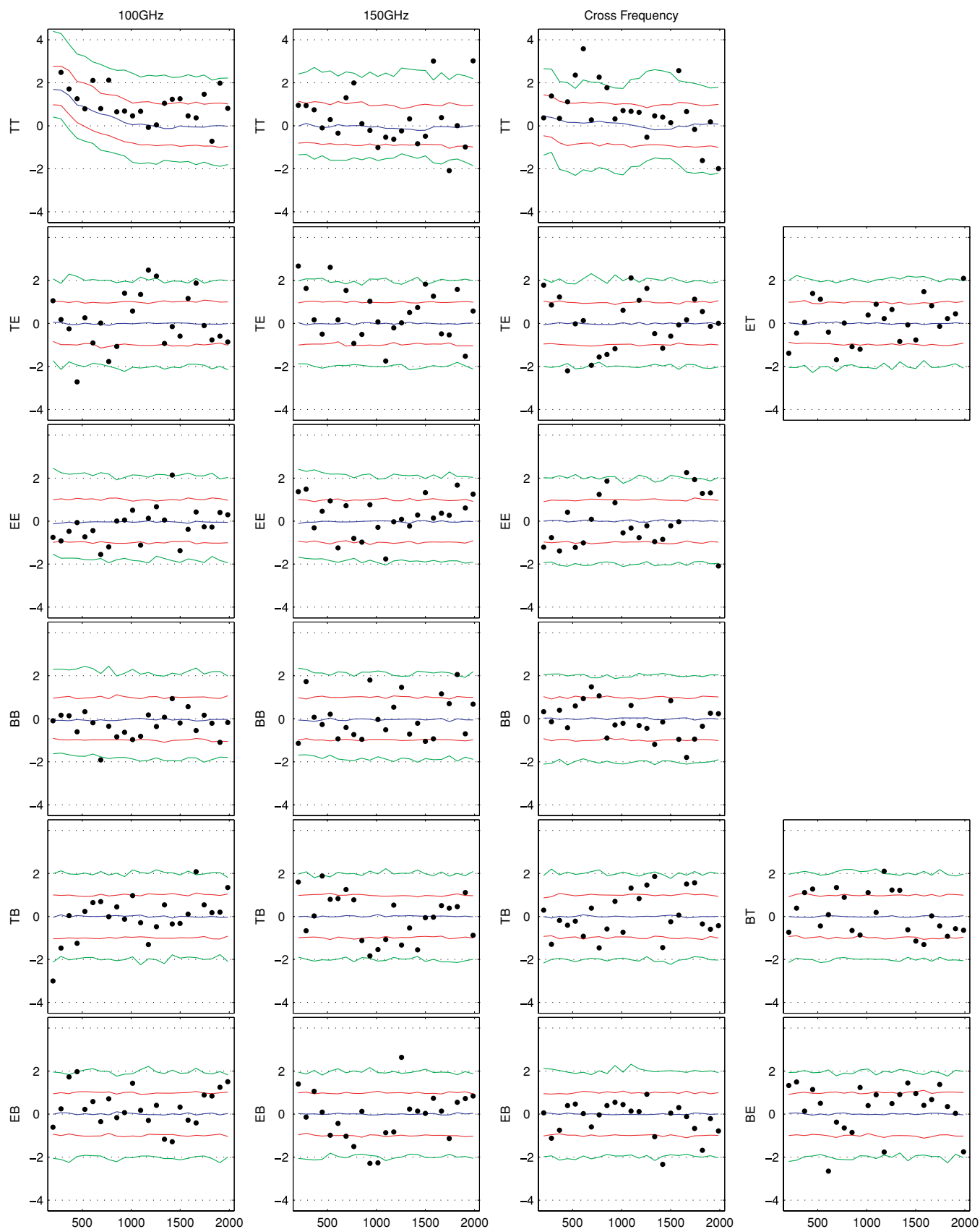
Figure 13. Bandpower deviations of the deck jackknife spectra. The horizontal axis is multipole number. The spectra shown as magenta points in Figure 11 have been divided by their error bars to investigate the contribution of each bandpower to \chi^2 . The green, red, and blue lines show the 2.3%, 15.9%, 50%, 84.1%, and 97.7% points of the integral distribution of the simulated signal plus noise bandpower values.
