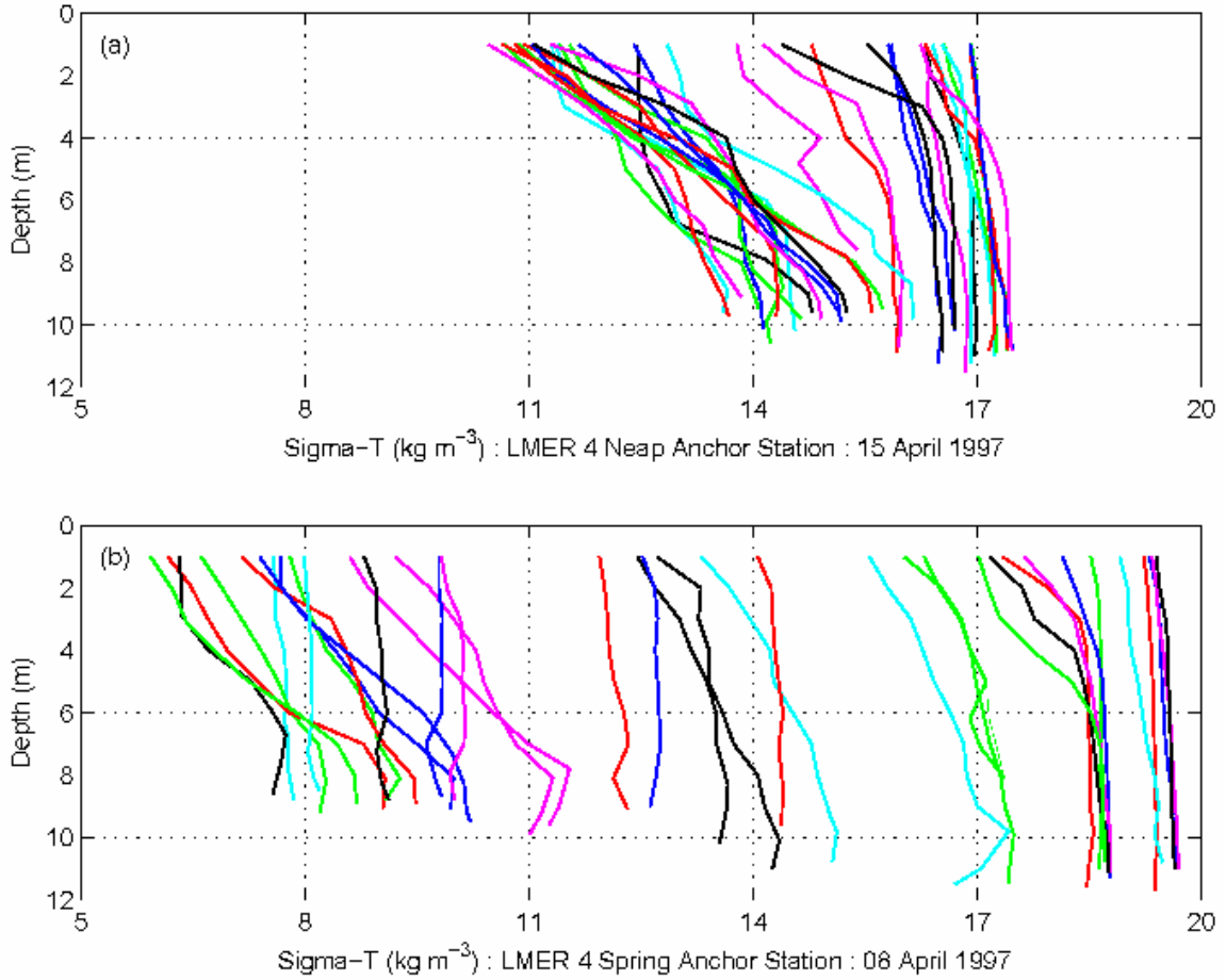
Figure 5.4: (a) Density profiles taken during the neap LMER 4 anchor station. The maximum vertical density difference observed during the neap anchor station was \Delta\rho = 5.1 \text{ kg m}^{-3} . (b) Corresponding density profiles taken during the spring LMER 4 anchor station. The maximum vertical density difference observed during the spring anchor station was \Delta\rho = 1.4 \text{ kg m}^{-3} . The different colors represent individual casts.
