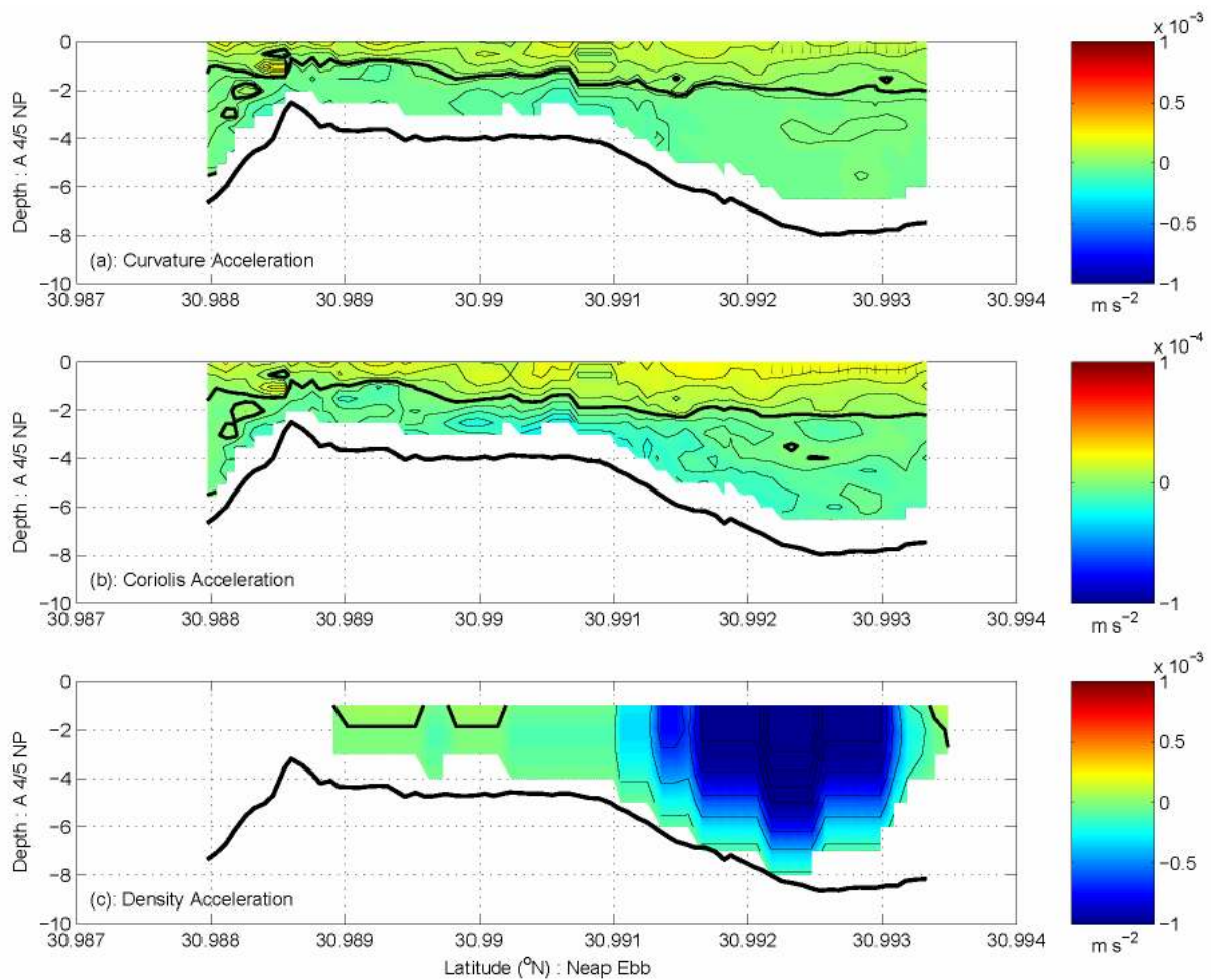
Figure 7.31: The (a) curvature acceleration, the (b) Coriolis acceleration, and the (c) density acceleration terms for the LMBM at section Domain A 4/5 for maximum ebb at neap tide. The solid black line in the subpanels indicates the zero crossing.
