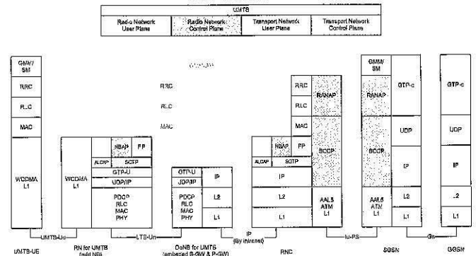
Figure 3. Protocol stack of control plane in Alt 1
