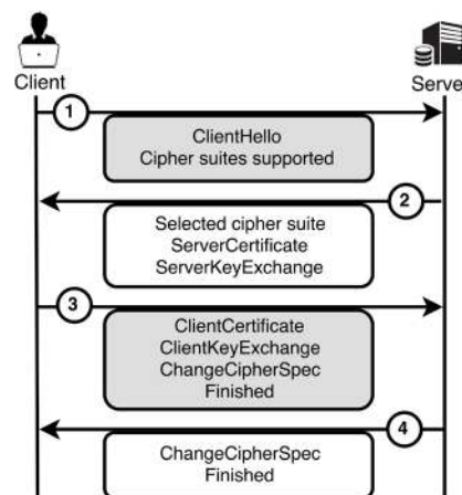
Figure 2. Illustration of TLS handshake process.
