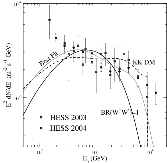
Fig. 4.— The HESS 2003 (grey squares) and HESS 2004 (filled circles) data on the flux of GR from the GC, and the best fit to those data with a KK B^{(1)} pair-annihilating lightest KK particle (dashed line), with a WIMP annihilating into a W^+W^- pair (black solid line), and with the best WIMP spectral function fit (light grey line).
