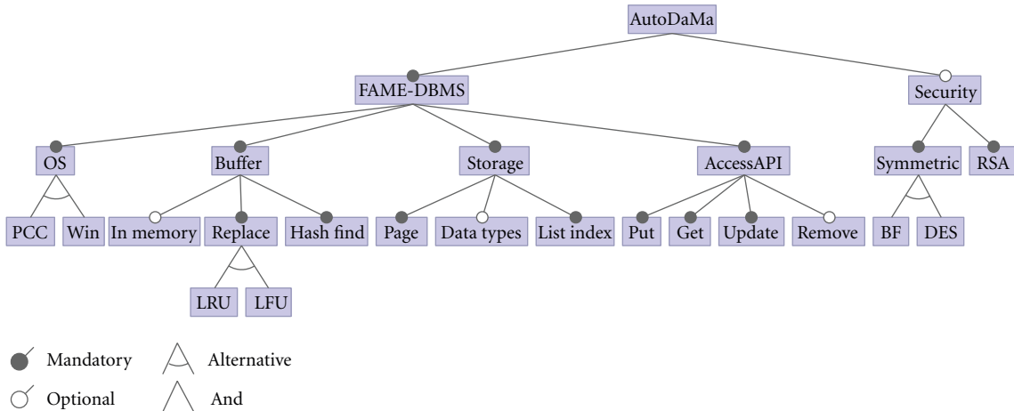
FIGURE 2: A feature model describing the valid feature combinations of AUTO DAMA. AUTO DAMA consists of the FAME-DBMS product line and some security-related features. Filled circles indicate mandatory features and empty circles optional features. An arc indicates that exactly one of the subfeatures is required, that is, the features are alternative to each other.
