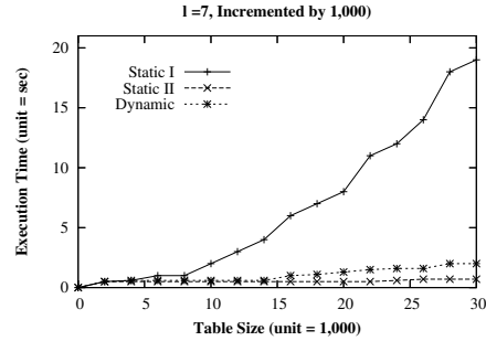
Fig. 11. Execution Time
