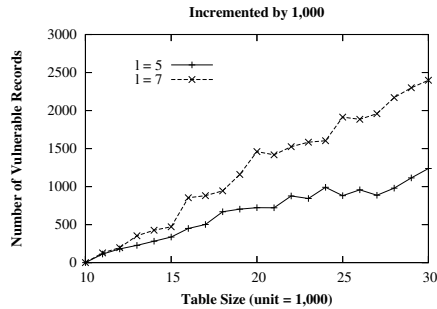
Fig. 8. Vulnerabilities
