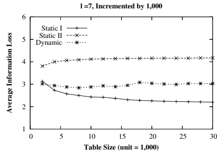
Fig. 9. Data quality
