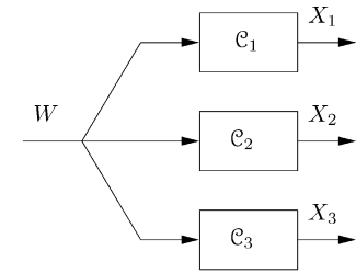
(a) Secrecy capacity-achieving code structure.
