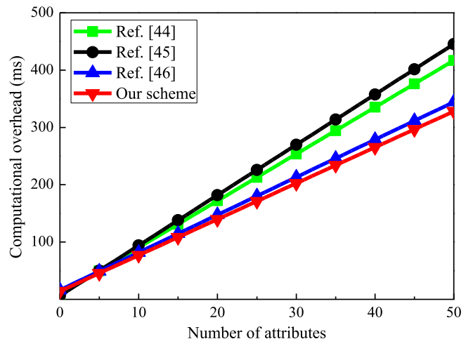
(b) Re-encryption
