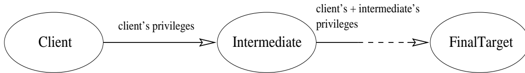
Figure 3: Delegation Chaining
