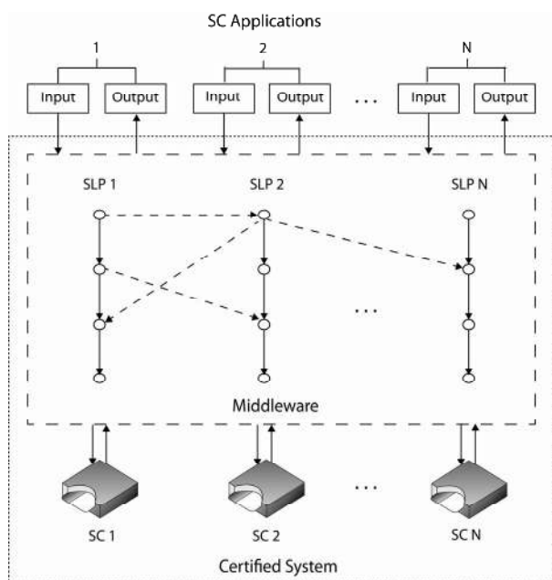
Figure 1. Middleware.
