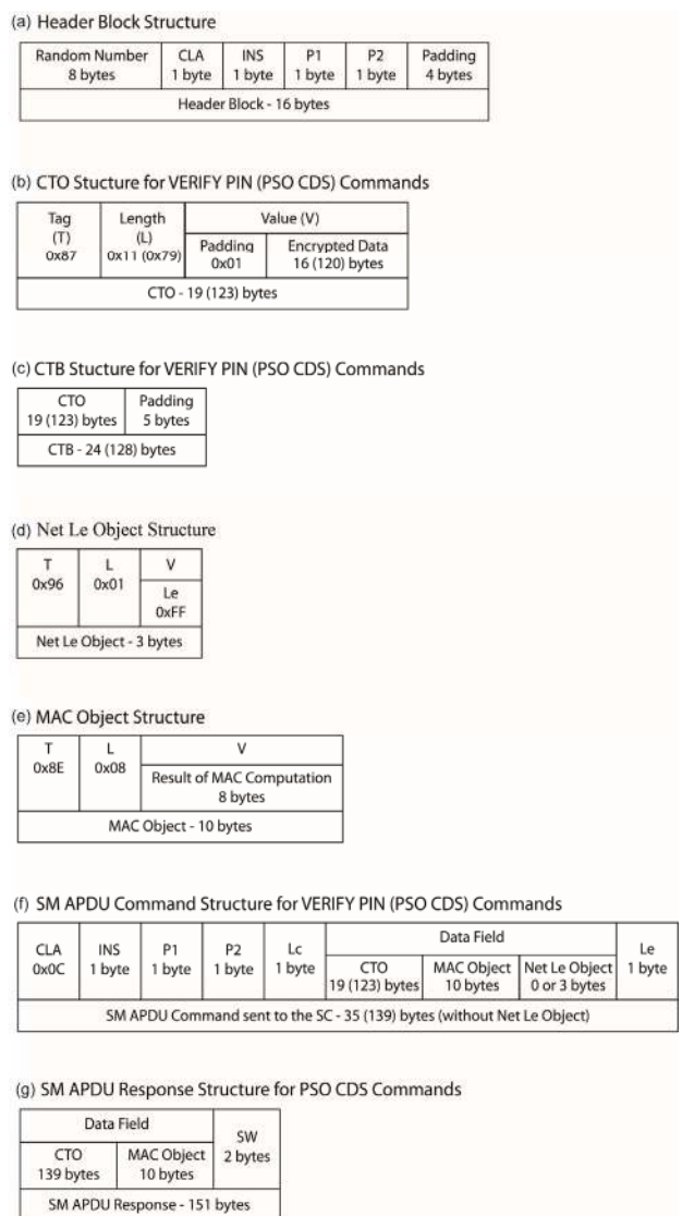
Figure 5. Structure of the objects in the SM operation.
