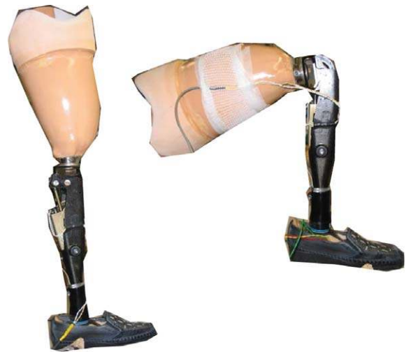
Fig. 2. The constructed prototype of the knee prosthesis.
