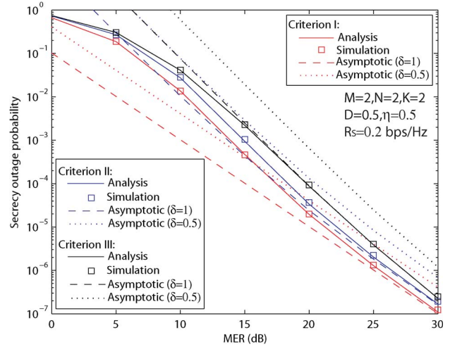
Fig. 2. Asymptotic secrecy outage probability versus MER.
