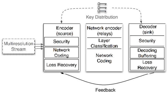
Fig. 6. Modules of a potential system implementation. Entities that are external to our system (that is, key distribution and generation of a multiresolution stream) are in dashed.
