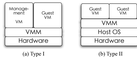
Figure 1. Types of virtualization architectures
