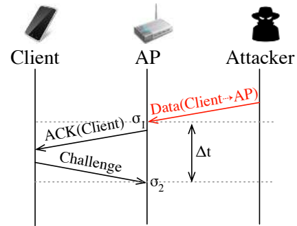
Figure 7: Authenticated spoofing attack and mitigation with DataCheck. Clients send protected minimal-length data frames or normal traffic in response to unexpected ACKs from the AP. The AP makes an AoA signature comparison between the attacker’s data frame ( \sigma_1 ) and the legitimate client’s subsequent challenge data frame ( \sigma_2 ).
