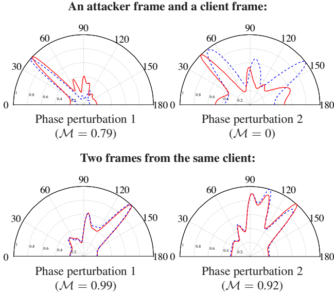
Figure 4: The effect of random phase perturbation on AoA signatures: Upper: comparison between an attacker’s frame and a client’s frame. Lower: comparison between two frames from the same client. \mathcal{M} is the similarity metric (§2.1.2).
