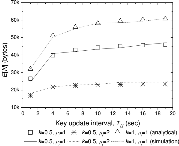
Fig. 5. The expected volume of exposed packets over the key update interval.
