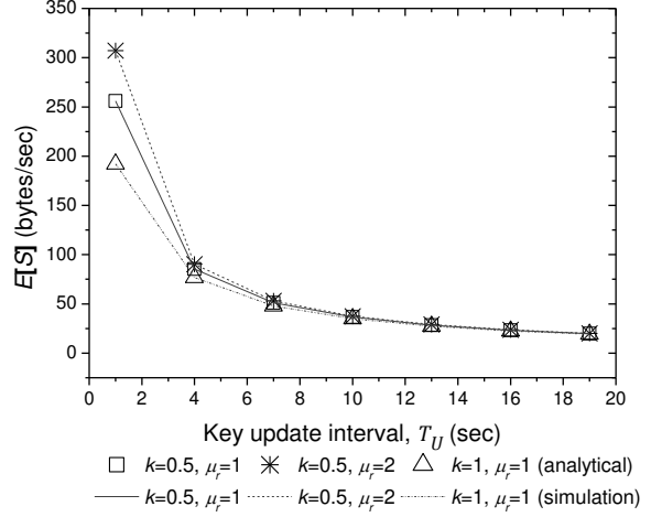
Fig. 6. The expected signaling overhead over the key update interval.
