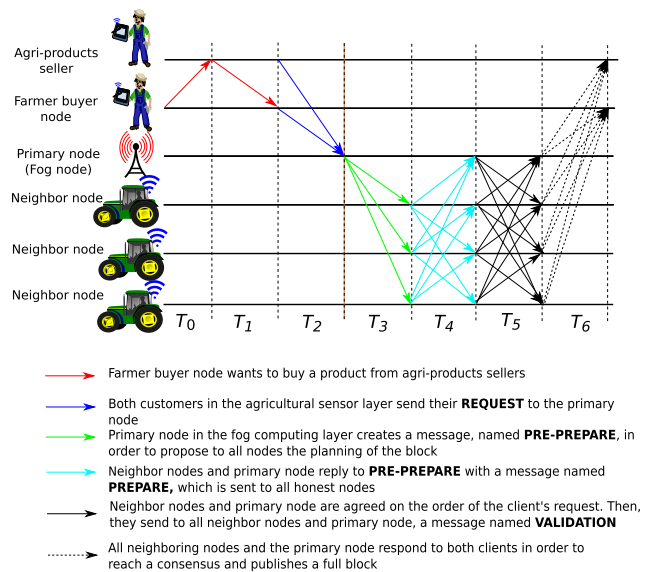
FIGURE 6. The consensus process based on the practical Byzantine fault tolerance (PBFT) algorithm for blockchain-based agri-products distribution.
