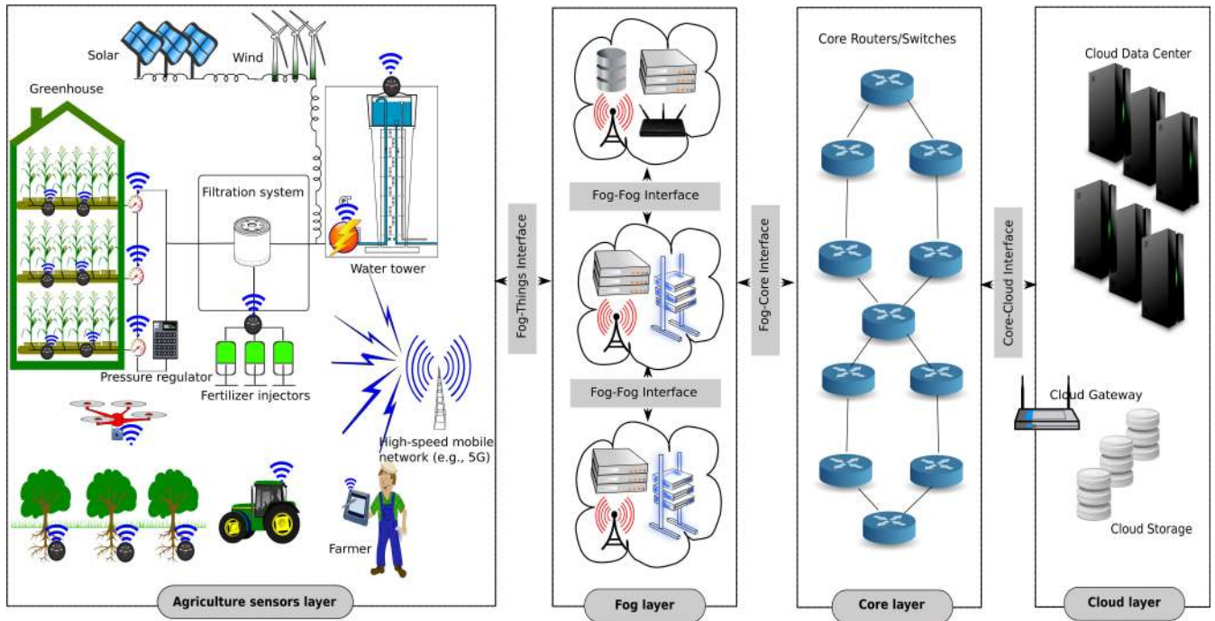
FIGURE 1. Four-tier green IoT-based agriculture architecture.
