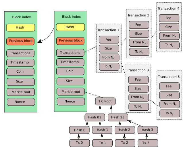
FIGURE 3. The blockchain data structure.
