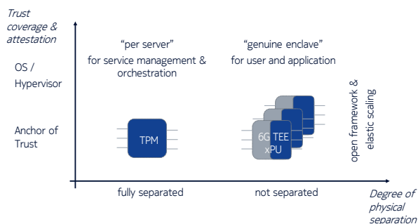
FIGURE 8. 6G ANCHORS OF TRUST, TRUSTED EXECUTION ENVIRONMENT AND TRUSTED PLATFORM MODULE
