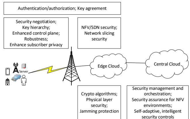
Fig. 4: Elements in a 5G security architecture [20]
