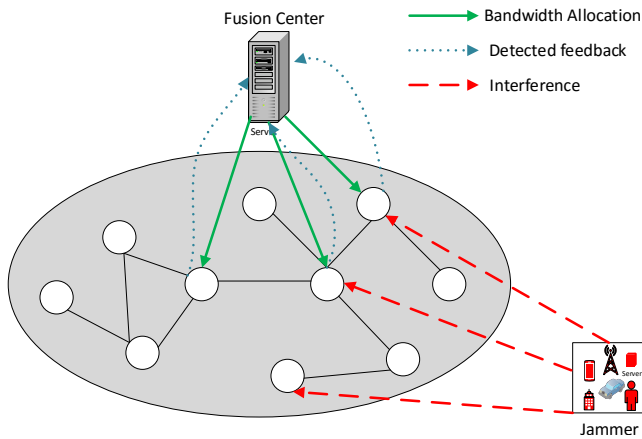
Fig. 11: The resource allocation model [40]
