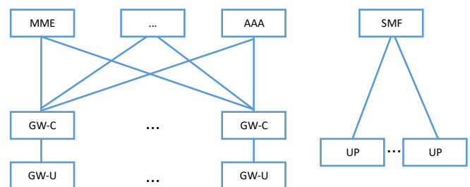
Fig. 22: Signaling architecture comparison of legacy cellular network and 5G cellular network
