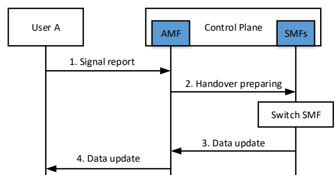
Fig. 21: A handover procedure for access technologies change
