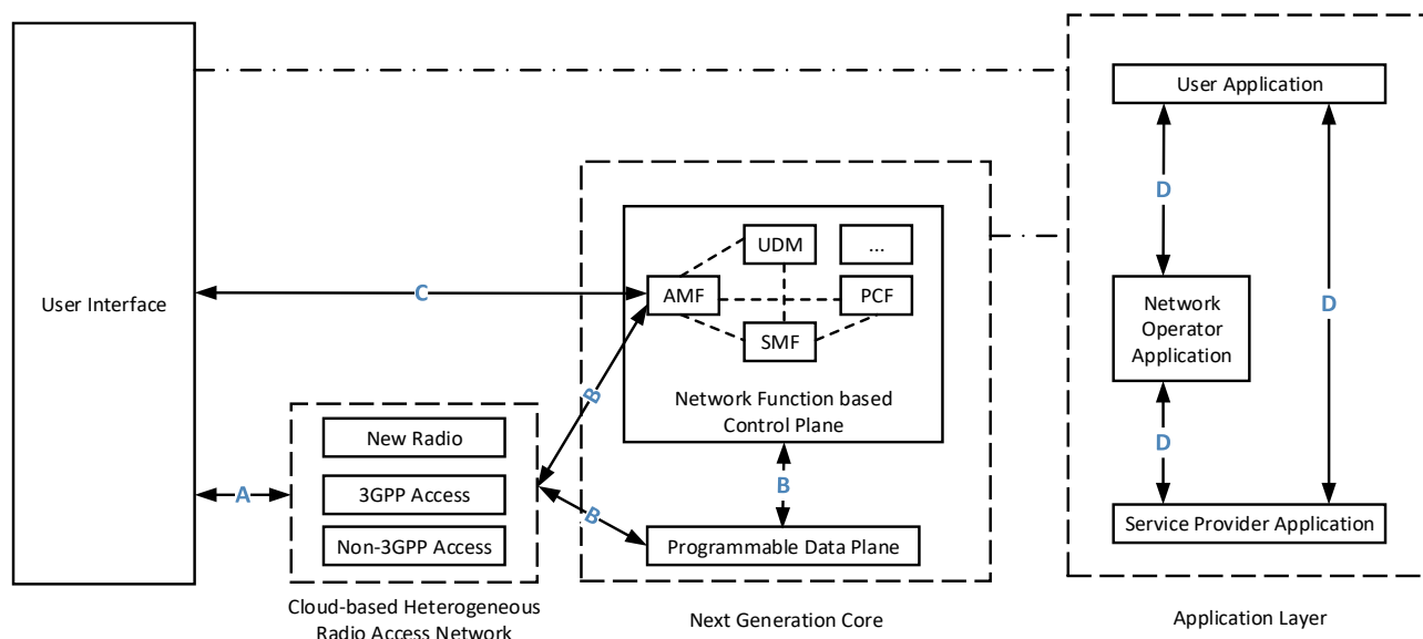
Fig. 16: The proposed 5G wireless network security architecture
