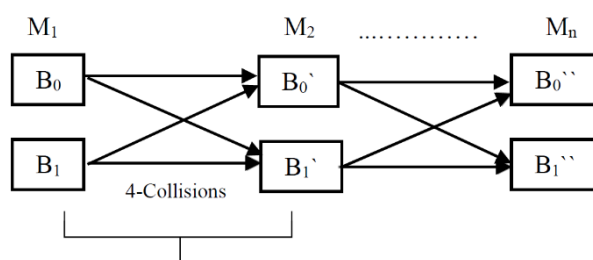
Figure 3. Multi-Collision attack
