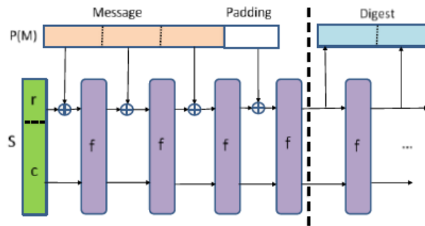
Figure 1. Sponge construction
