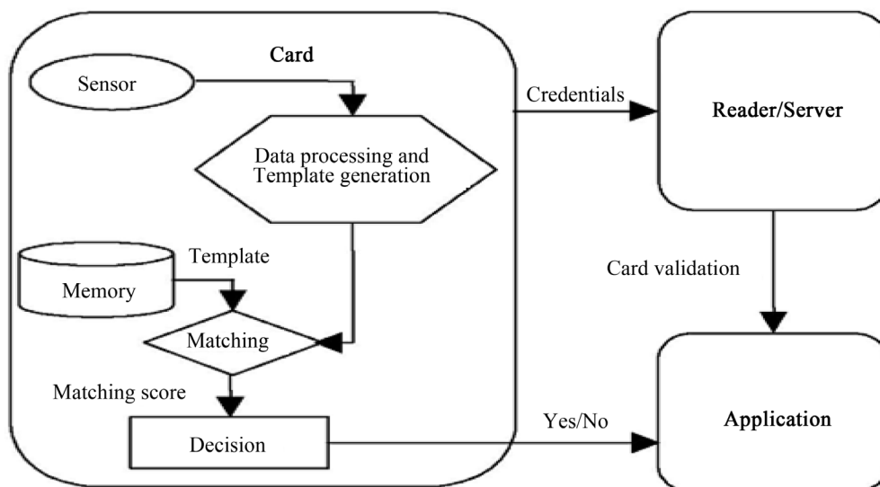
Figure 2. Biometric template-on-card and matching-on-card [19].
