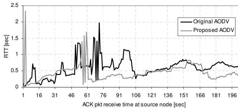
Figure 3: Acknowledgement packet receive time versus round trip time
