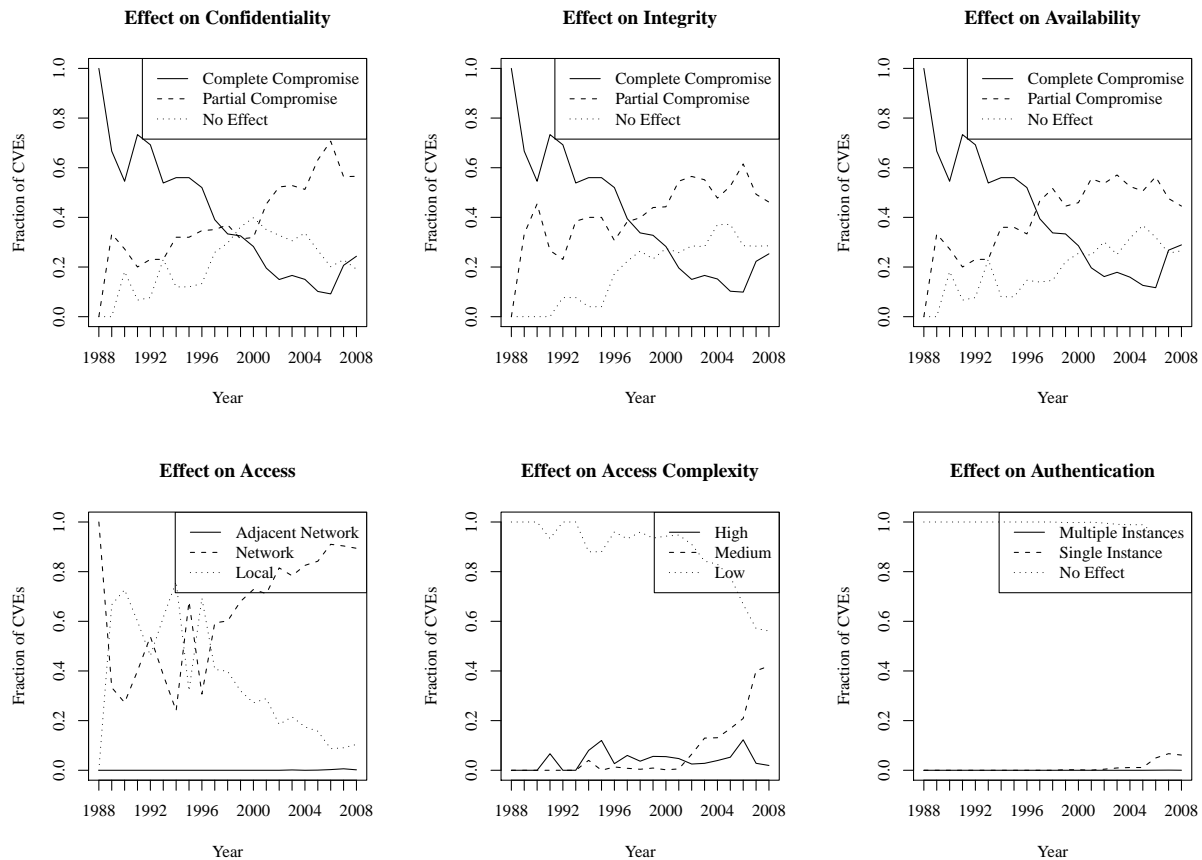
Figure 4. Development of CVSS impact vectors until 2009.
