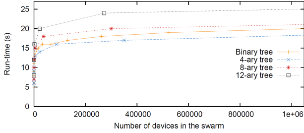
Figure 8: Performance of SEDA for tree topologies
