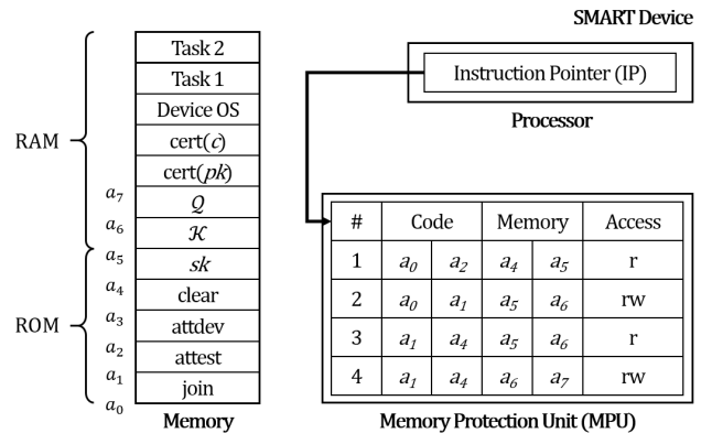
Figure 4: Implementation based on SMART [16]
