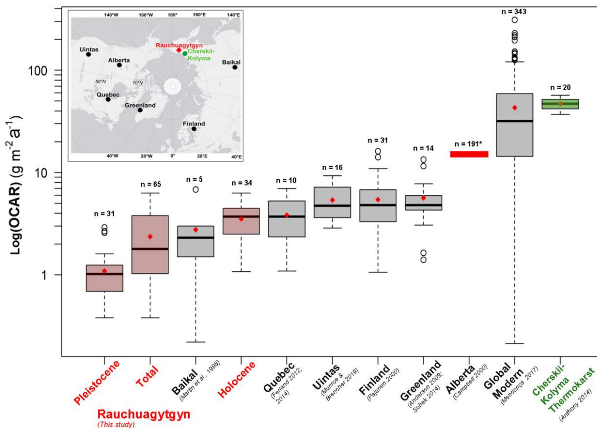
Figure 8. Comparison Log-boxplot of average organic carbon accumulation rates (OCARs) for Lake Rauchuagytygn with carbon accumulation rates from other regions. Rauchuagytygn OCARs include a total of 65 downcore points and plot close to Boreal lake sites and to Lake Baikal (ESRI 2020). The global modern dataset of Mendonça et al., 2017 included OCARS from 343 globally distributed lake sites (see Text S1). Study references are quoted below the study regions.
