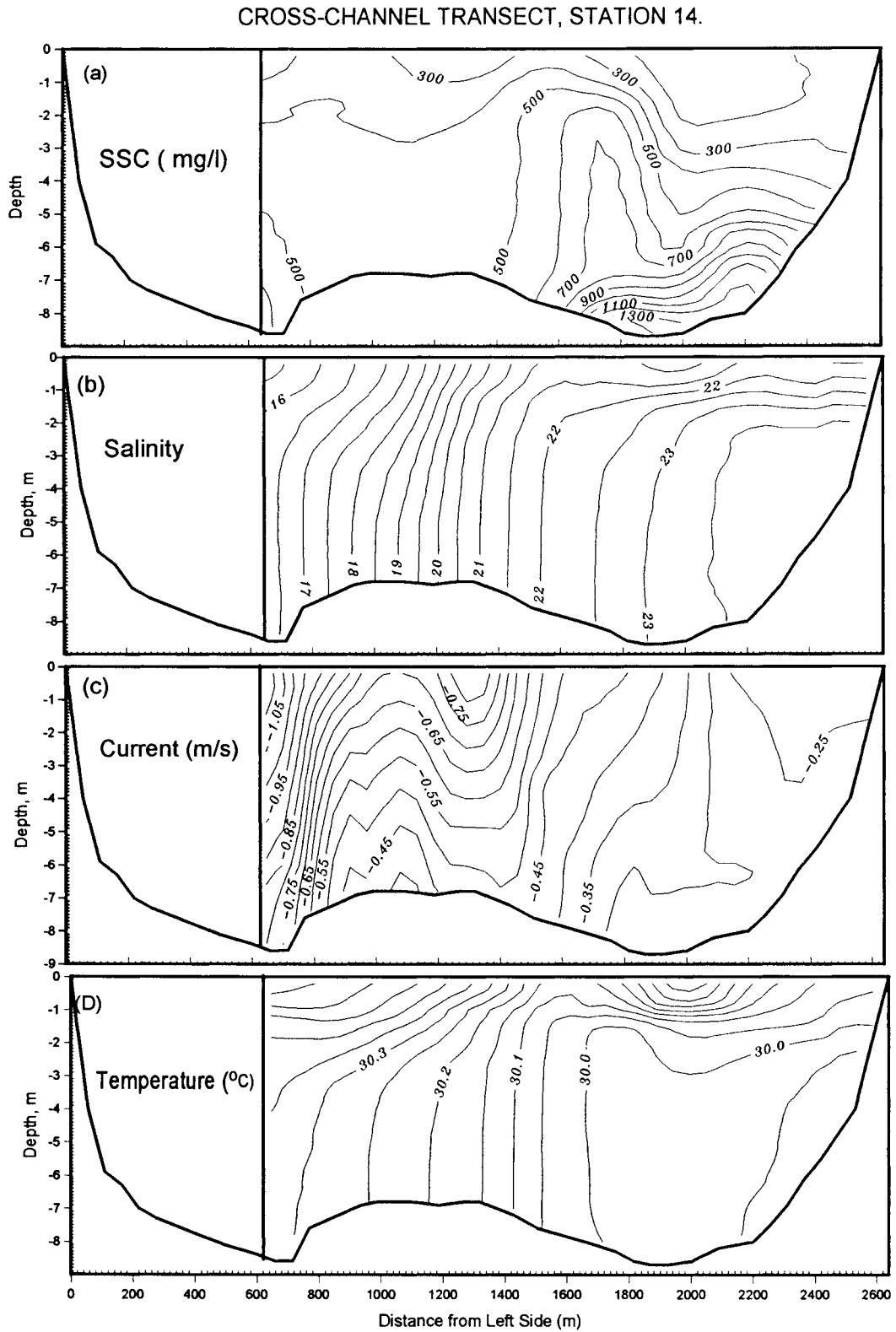
Figure 7. Cross-sectional distribution of suspended sediment concentration (SSC, in \text{mg l}^{-1} or \text{g m}^{-3} ), salinity, currents and temperature along a transect past station 14, 1400–1600h, April 16, 1996.
