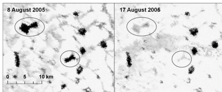
Fig. 9. Remotely sensed spatial distribution (MODIS bands 1, 1, 2 = RGB) of supraglacial lakes within the 15 000 km 2 ice-sheet area (Fig. 1) on 8 August and 17 August in 2005. Several lakes remain intact between 8 and 17 August, except for two lakes ~11 km 2 (red circles) that drained.
