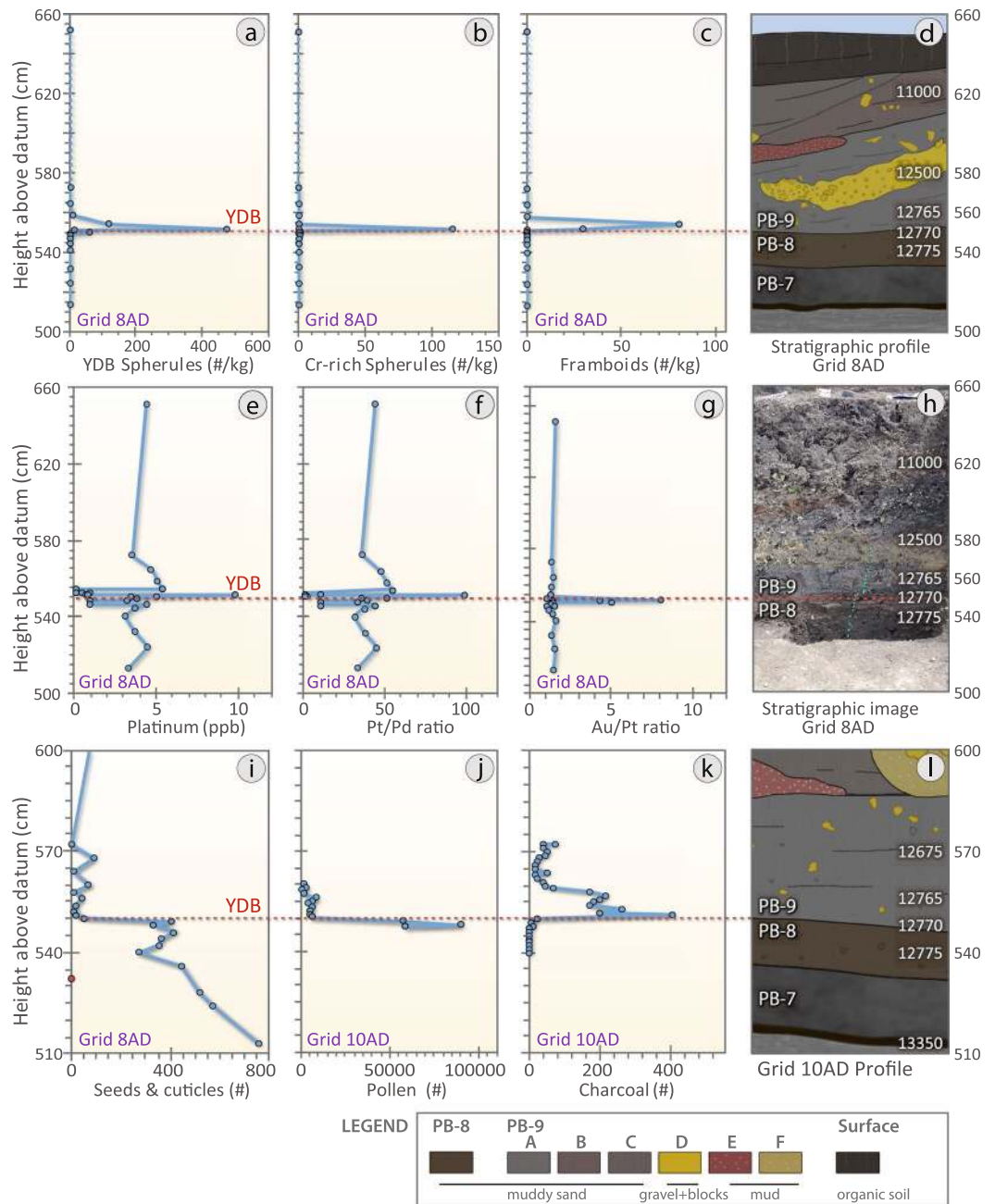
Figure 4. Changes in impact-related and environmental proxies at the PB-8/PB-9 boundary (YDB), showing peak concentrations of high-temperature impact spherules, frambooids, and elemental proxies, including Pt, along with changes in charcoal and plant macrofossil abundances. (a) Group 1: high-temperature, Fe- and Si-rich impact spherules exhibit a peak abundance of ~520/kg at ~552 cm; (b) Group 2: Cr-rich spherules have a peak abundance of ~115/kg at ~552 cm; (c) Group 4: authigenic frambooids have a peak abundance of ~80/kg at ~554 cm. (d) Stratigraphic profile of grid 8AD. Age of PB-8/PB-9 boundary is 12,770 \pm 160 cal yr BP. (e) Pt abundance peak of 9.9 ppb in the YDB layer at 551 cm coincident with the boundary of units PB-8 and PB-9. (f) Anomalous Pt/Pd ratios are restricted to the PB-8/PB-9 boundary suggesting the influx of non-local Pt at the YDB. (g) Anomalous Au/Pt ratios are also restricted to the PB-8/PB-9 boundary suggesting the influx of non-local Au at higher concentrations than those of the non-local Pt. (h) Photograph of sampling section in grid 8AD. Green pins mark sampling levels. (i) Abundance record of seeds showing the major decline at the YDB layer. (j) Pollen concentrations showing the abrupt decline in the YDB layer. (k) Abrupt increase in charcoal peaking at the YDB layer with continuing high concentrations in the overlying ~10 cm. (l) Stratigraphic profile for grid 10AD. Group 3 volcanic spherules were found in low concentrations throughout the profile in grid 8AD (not plotted here; see Supplementary Fig. S11a). Group 5 anthropogenic spherules were restricted to surface sediments in grid 8AD (not plotted here; see Supplementary Fig. S11b). Group 6 rounded detrital grains (not plotted) are common throughout the entire profile. Legend is the same as in Fig. 2.
