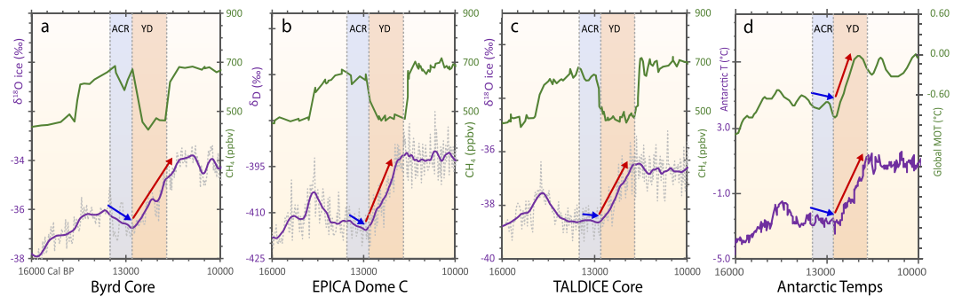
Figure 14. Antarctic climate record exhibiting warming trend at ~12,800 cal BP. Changes in methane ( \text{CH}_4 ) concentrations are used to identify and correlate climate change boundaries representing the Antarctic Cold Reversal and the Younger Dryas. Climatic history is reflected by changes in \delta^{18}\text{O} and \delta\text{D} values, which are proxies for temperature, with lower values indicating cooler climate. (a) Byrd core in West Antarctica; (b) EPICA Dome C near the center of East Antarctica; (c) TALDICE core from Talos Dome in southern East Antarctica; (d) green upper curve represents global mean ocean temperature from WAIS divide near Byrd in West Antarctica. Purple lower curve represents atmospheric temperatures reconstructed from \text{CO}_2 record at EPICA Dome C 140 . Blue vertical bar represents cooler climate during the Antarctic Cold Reversal, anti-phased with the warm Bølling-Allerød episode in the Northern Hemisphere. Orange vertical bar represents warmer climate in Antarctic coeval with Younger Dryas cooling in the Northern Hemisphere. Blue and red arrows indicate colder or warmer temperature changes, respectively, across the Antarctic Cold Reversal and the Younger Dryas.
