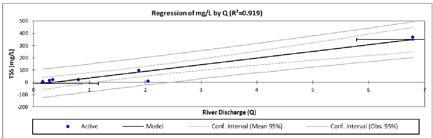
Fig. 6 The Regression of Total Suspended Sediment (TSS) and River Discharge (Q)
