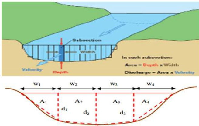
Fig. 3 The theoretical of discharge measurement by cross-section of the river
