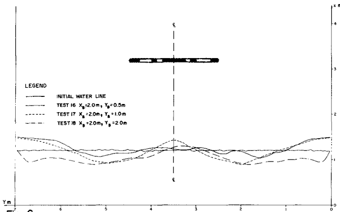
Fig. 6- WATER LINES IN EQUILIBRIUM STATE FOR TESTS SERIES H_0/L_0=0.040
