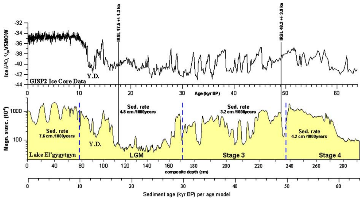
Fig. 3 The magnetic susceptibility of the upper 300 cm of the cores from Lake El'gygytyn is tuned against the \delta^{18}\text{O} from the GISP2 record (Grootes et al. 1993; Nowaczyk et al. 2007). IRSL ages calculated for the core has been added as additional chronology controls. The depth scale of the magnetic record is shown with sediment age given
